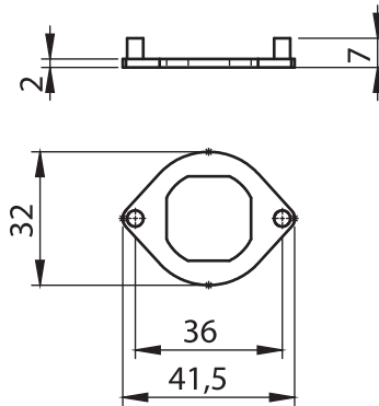
2900-407 - Fixing Adapter
