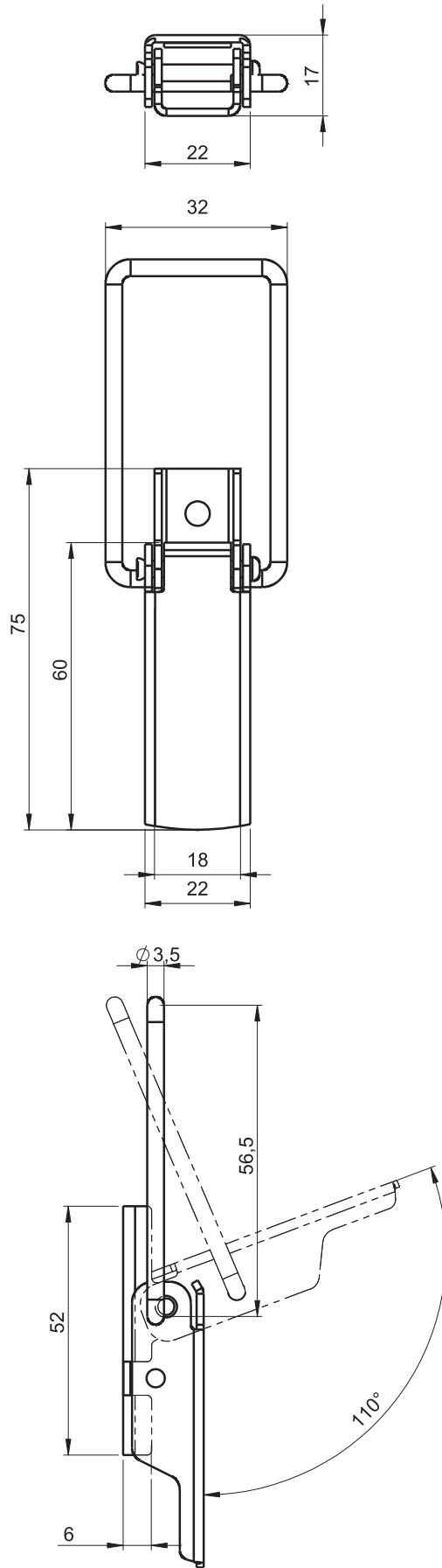
7404 - Toggle Latch
